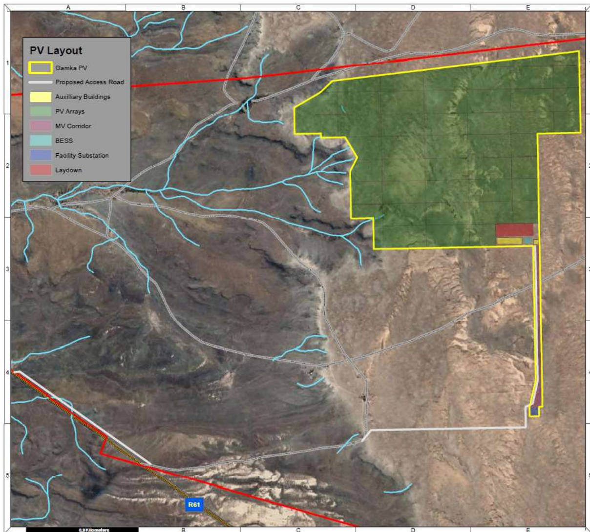
Figure 2: Proposed layout of Gamka PV, showing key project components (Please also refer to the full-scale plans attached in Appendix A).
