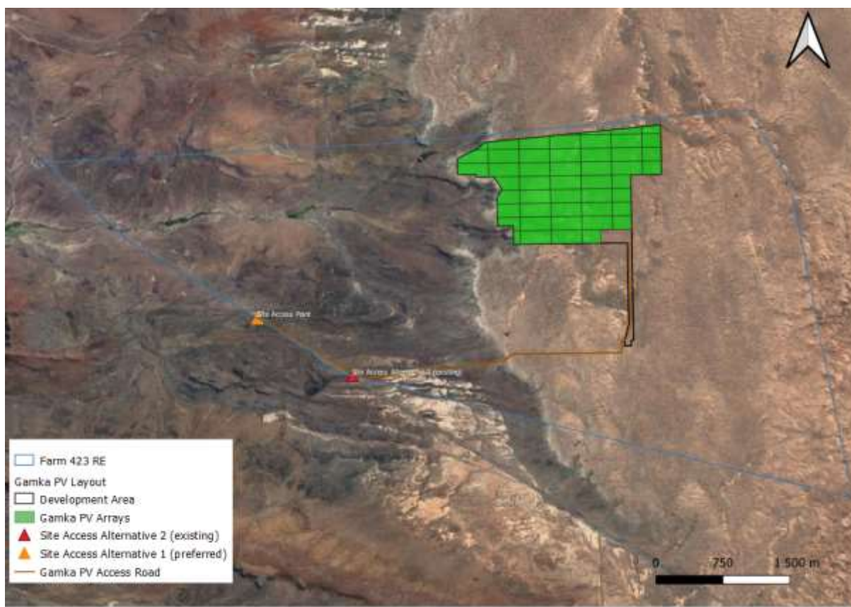
Figure 13: Access route and proposed access point to Gamka PV. Site Access 1 is the preferred access as identified in the Traffic Impact Assessment (Appendix E13)
