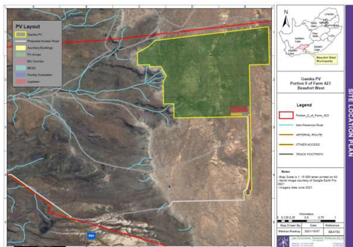
Figure 28: Layout Alternative 1 (preferred) for Gamka PV.
