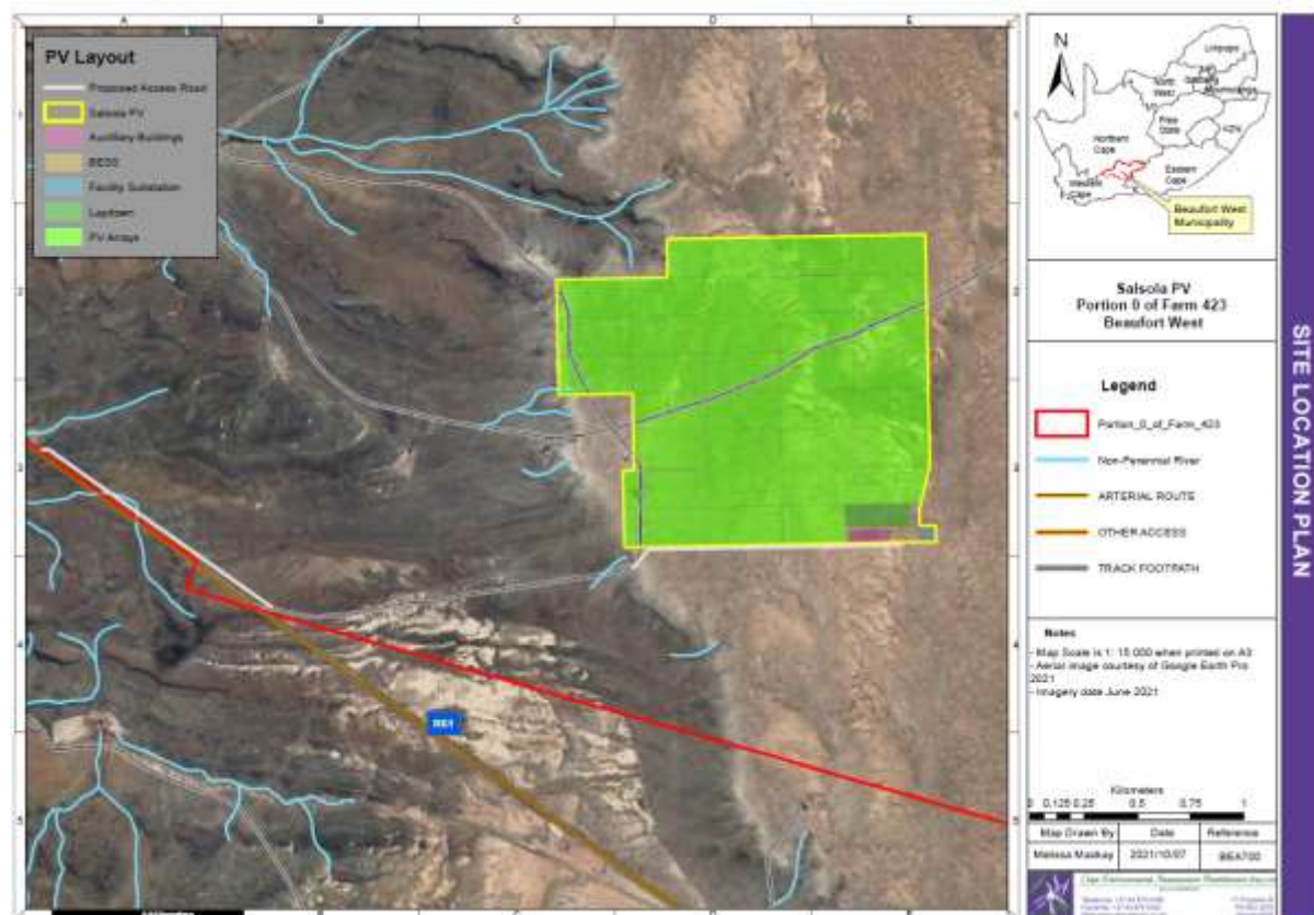
Figure 28: Layout Alternative 1 (preferred) for Salsola PV.
