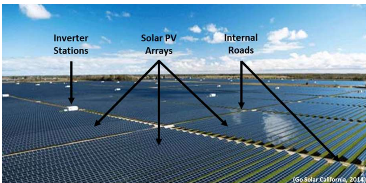
Figure 3: Typical configuration of a Solar PV Energy Facility (Salsola PV (Pty) Ltd)
