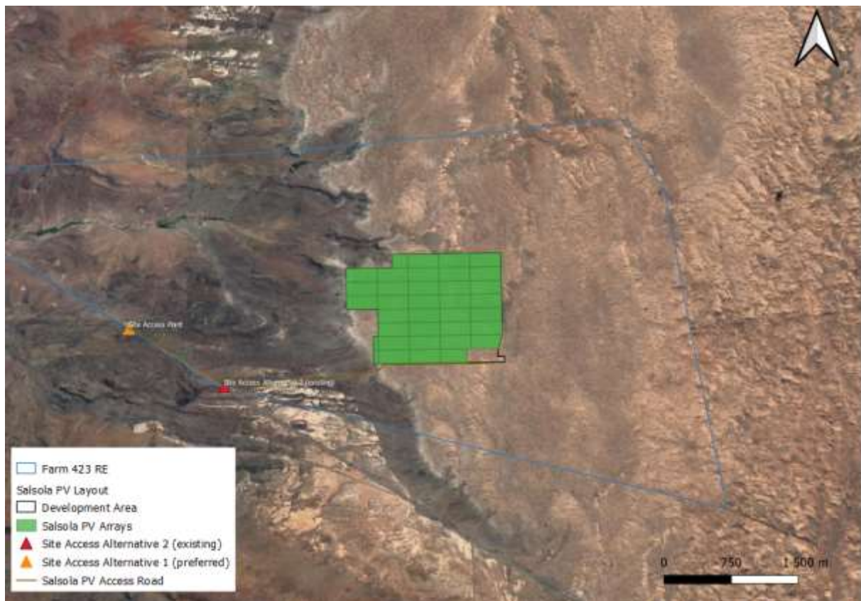
Figure 13: Access route and proposed access point to Salsola PV. Site Access 1 is the preferred access as identified in the Traffic Impact Assessment (Appendix E13)
