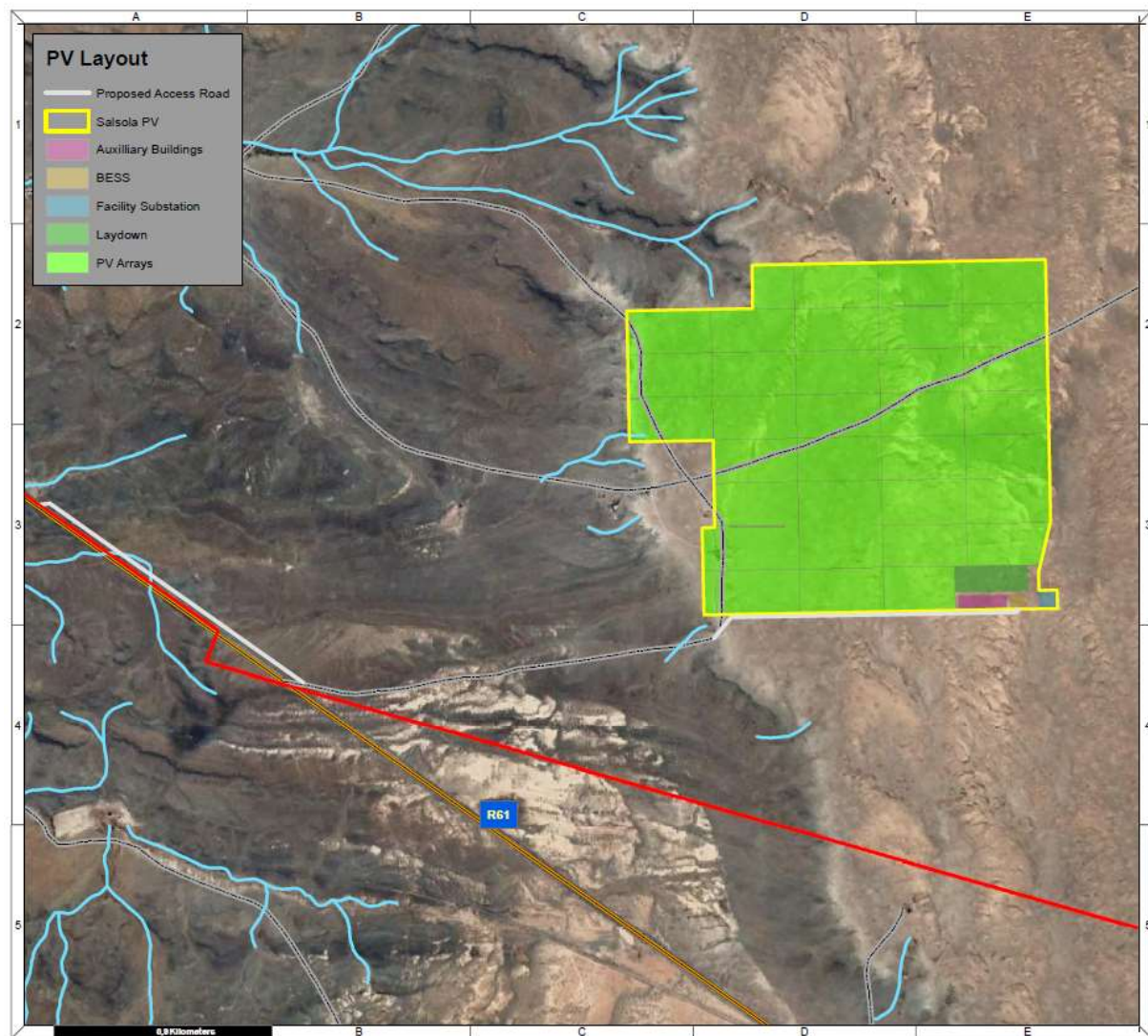
Figure 2: Proposed layout of Salsola PV, showing key project components (Please also refer to the full-scale plans attached in Appendix A).
