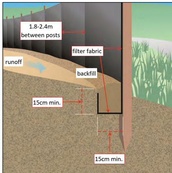
FIGURE 3-3: TYPICAL SILT FENCE (AFTER ENVIRONMENT PROTECTION AGENCY 4 )
