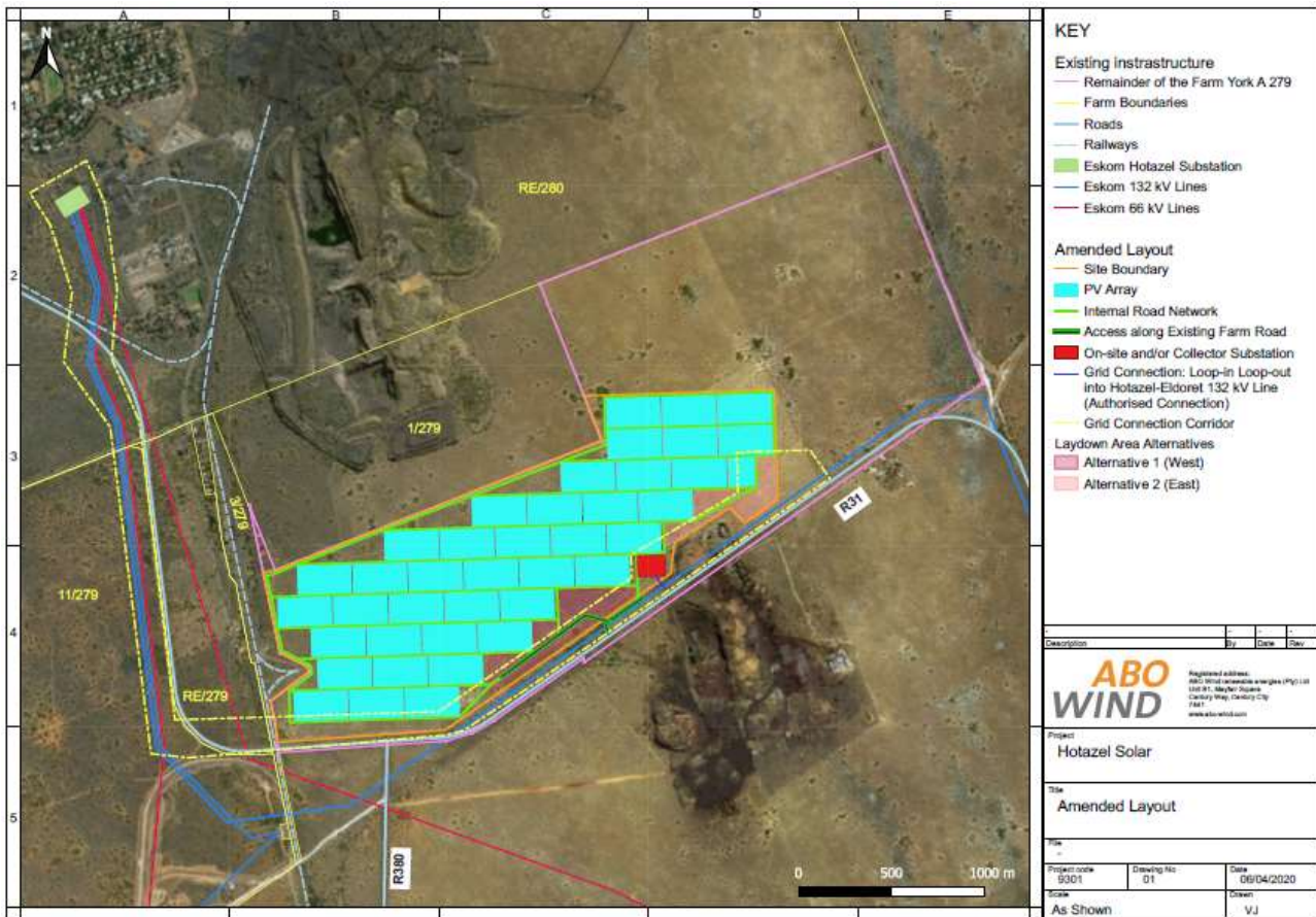
Figure 3: The location of the amended Hotazel Solar facility on the western half of the property.
