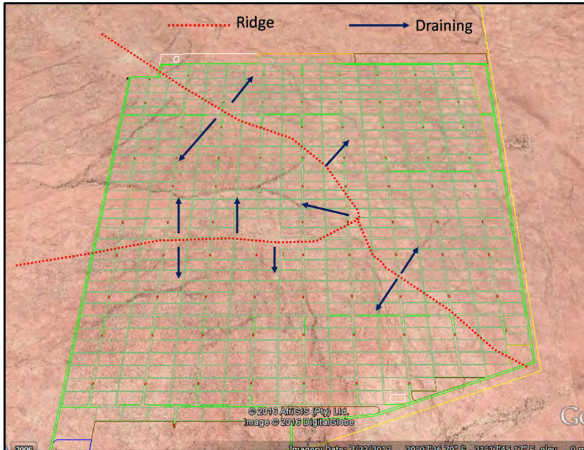
Figure 8: Drainage pattern
