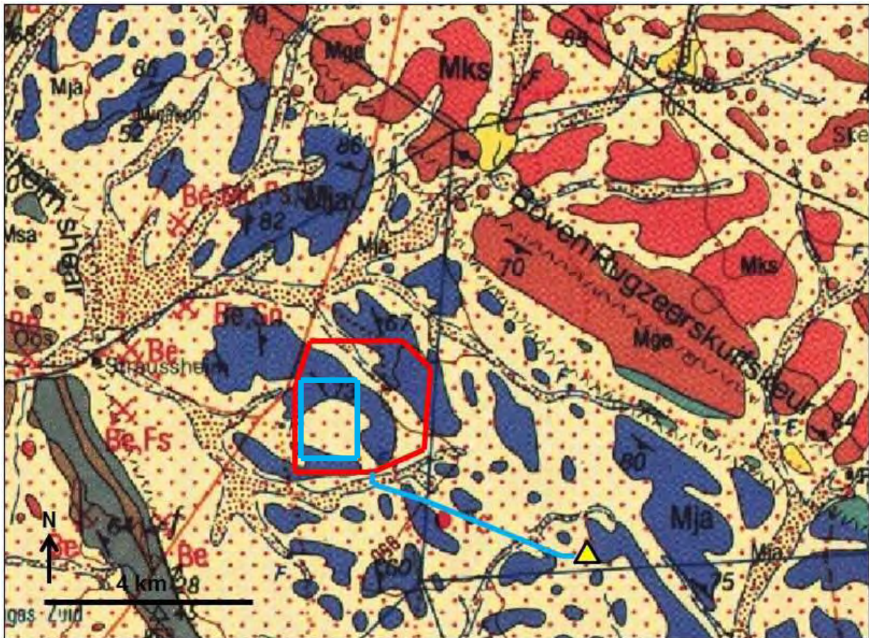
Figure 3. Figure 1. Extract from 1: 250 000 scale geological map sheet 2920 Kenhardt (Council for Geoscience, Pretoria) showing the geology of the AMDA Bravo Solar PV Development study area (blue rectangle) on Portion 1 of N'Rougas Zuid No 121, c. 30 km northeast of Kenhardt, Northern Cape. The pale blue line shows the proposed route of the 132 kV transmission line connection to the Nieuwehoop MTS Substation on Gemsbok Bult 120 (yellow triangle). The study area is underlain by Precambrian bedrocks of the Sandnoute Formation (Jacomyns Pan Group) (Mja, blue). The bedrocks are overlain in many areas by aeolian sands of the Gordonia Formation (Kalahari Group) (Qg, pale yellow with sparse red stipple) and Late Caenozoic alluvium (sands & gravels) (pale yellow with dense stipple).
