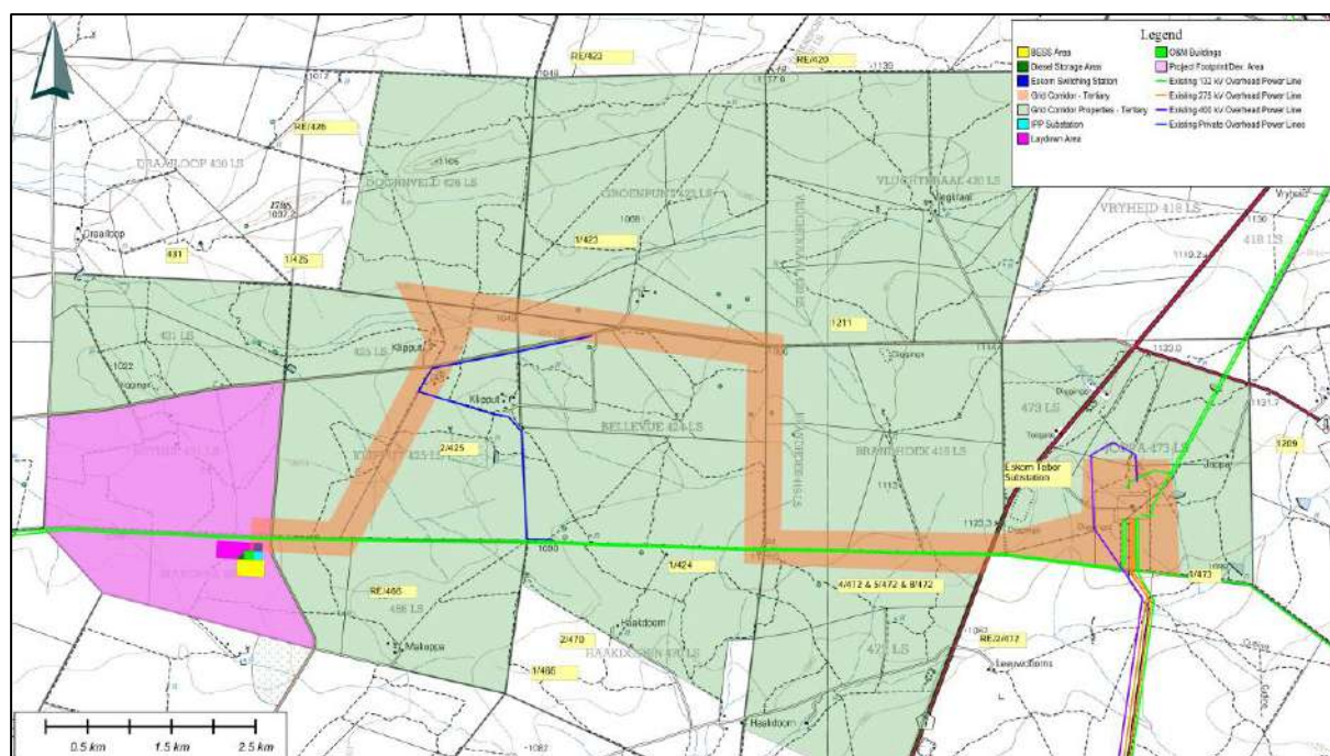
Figure 31: Grid Connection Alternative 3.
