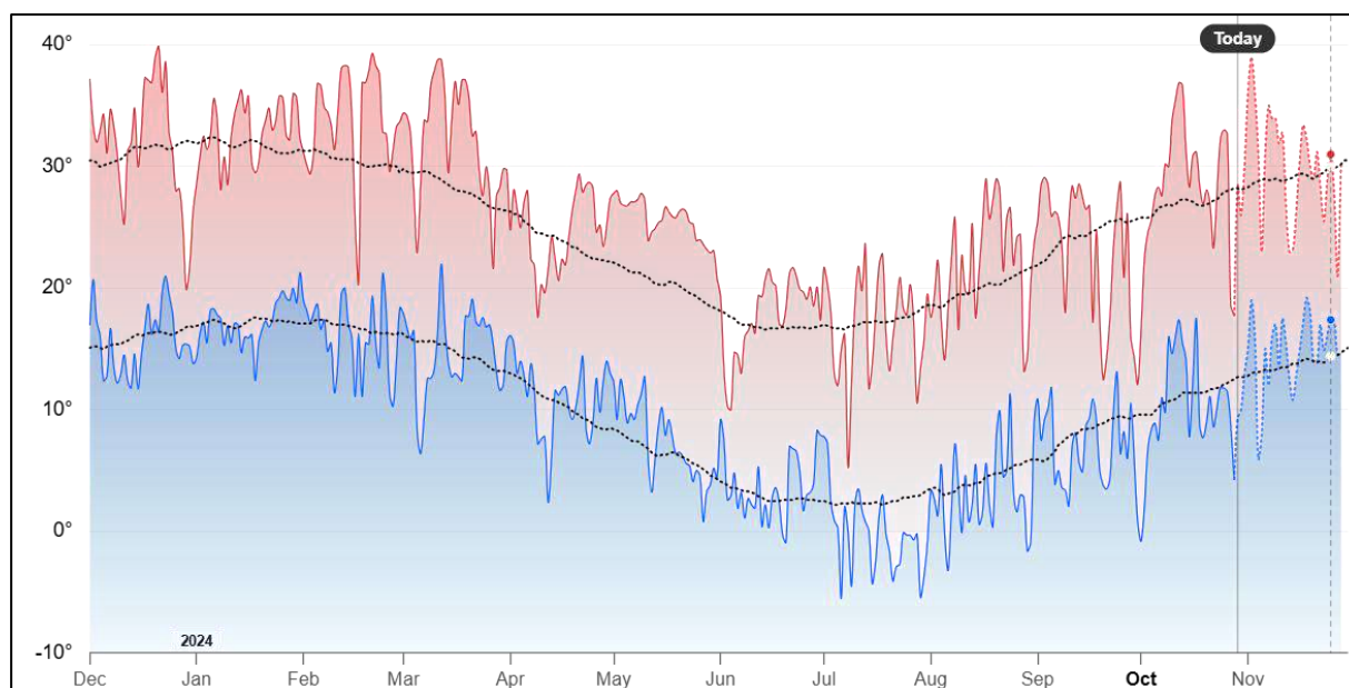
Figure 40: Average Monthly Temperatures for the Louis Trichardt Area.
