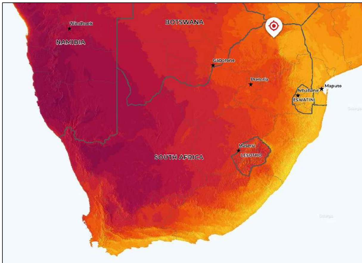
Figure 21: Global Horizontal Irradiation of the Bethel Solar PV (Solar Atlas, 2025).
