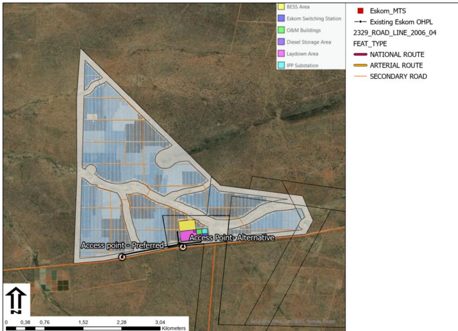
Figure 7: Proposed Draailoop Solar PV and associated infrastructure assessment areas map.
