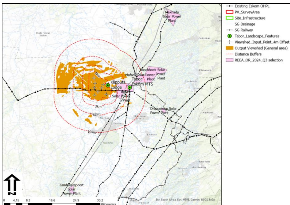
Figure 12: Map depicting DEA Renewable Energy project status in relation to the preliminary viewshed generated from the site highpoints for Draailoop Solar PV project (4m Offset).
