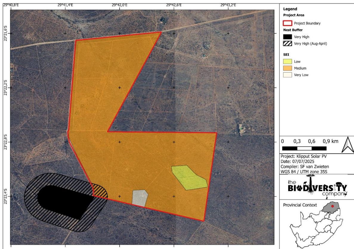
Figure 3-24 Site ecological importance, with mitigation measures applied
