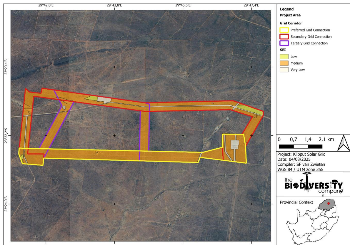
Figure 3-24 Site ecological importance, with mitigation measures applied
