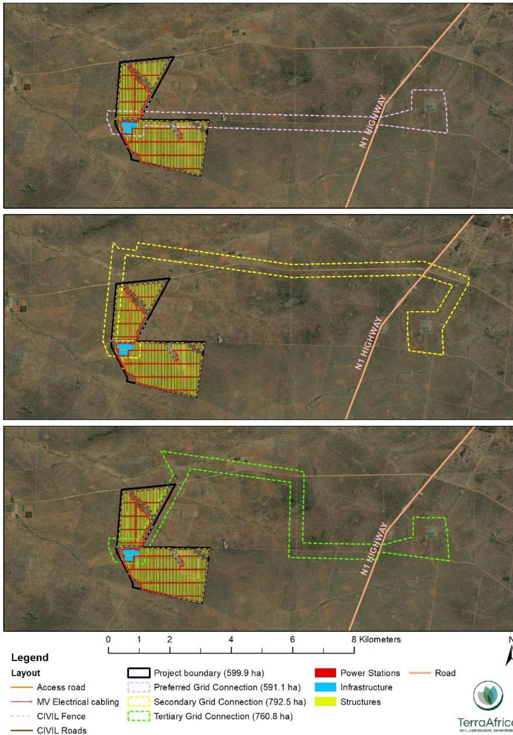
Figure 2: Layout map of the Klipput Solar PV project and alternative locations of the grid connection corridor
