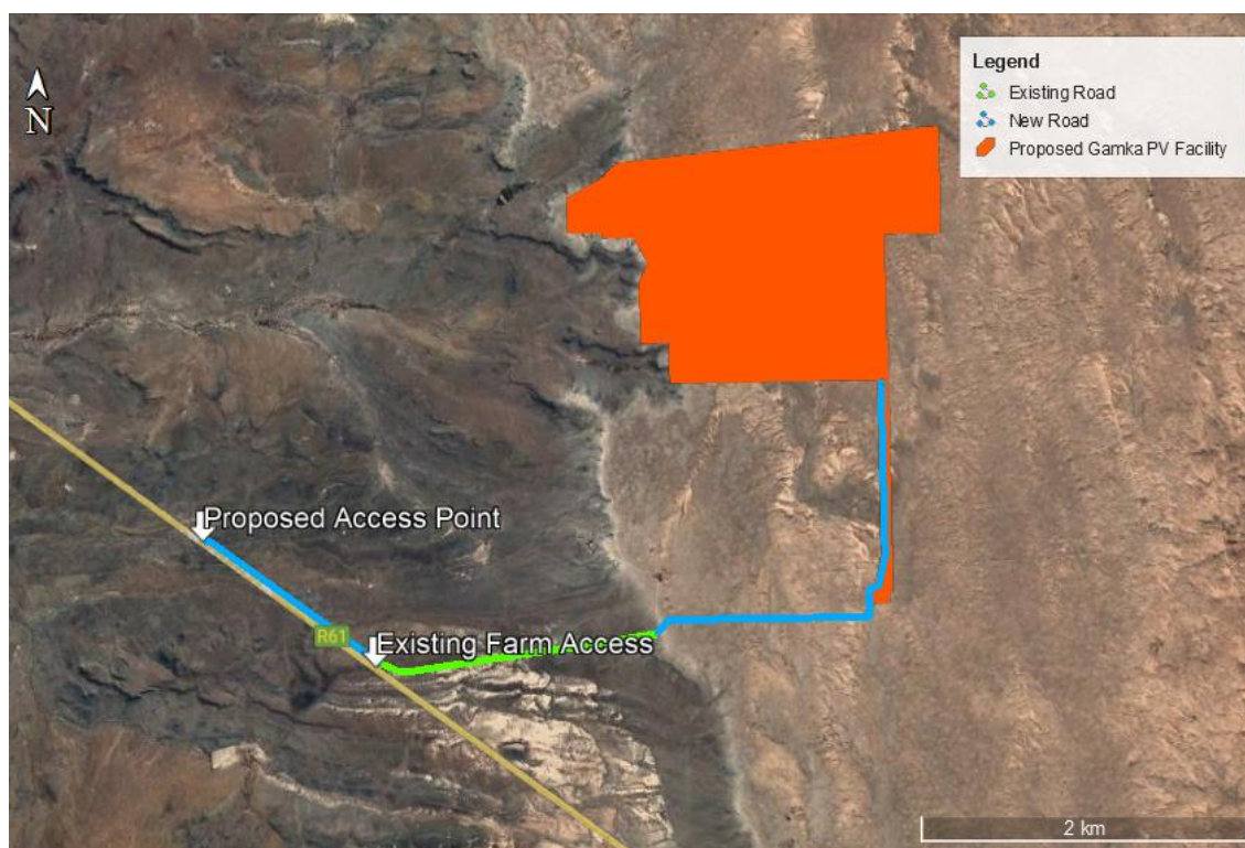
Figure 3-6: Proposed Access Road and Proposed Access Point
