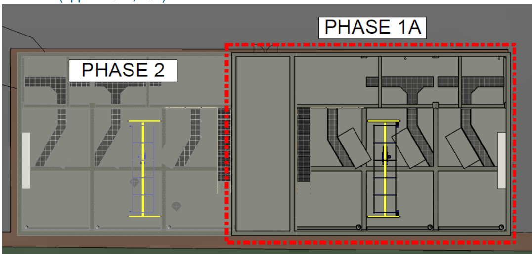
Figure 40: Concept pumpstation layout (Phase 1A and 1B)
