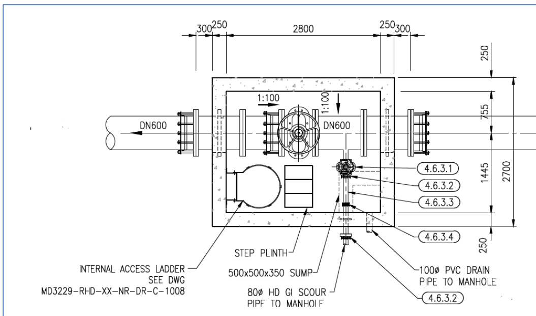
Figure 36: Sectional view of reservoir outlet chamber
