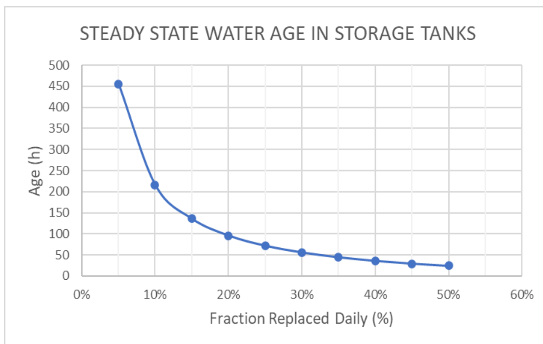
Figure 3 : Steady State Water Age in storage Tanks
