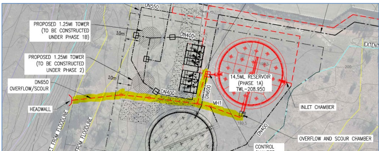
Figure 39: Preliminary drainage pipe route from overflow and control chambers to discharge point (route highlighted)
