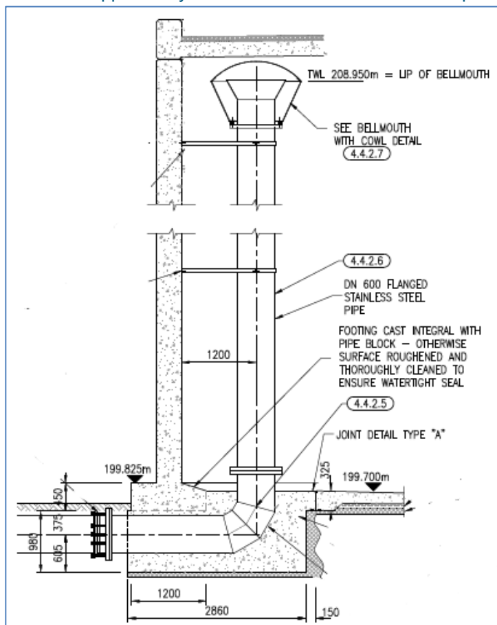
Figure 37: Preliminary detail for emergency overflow
