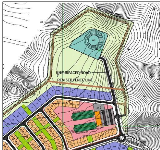
Figure 5 – Hartenbos Garden Estate Site Development Plan in vicinity of reservoir
