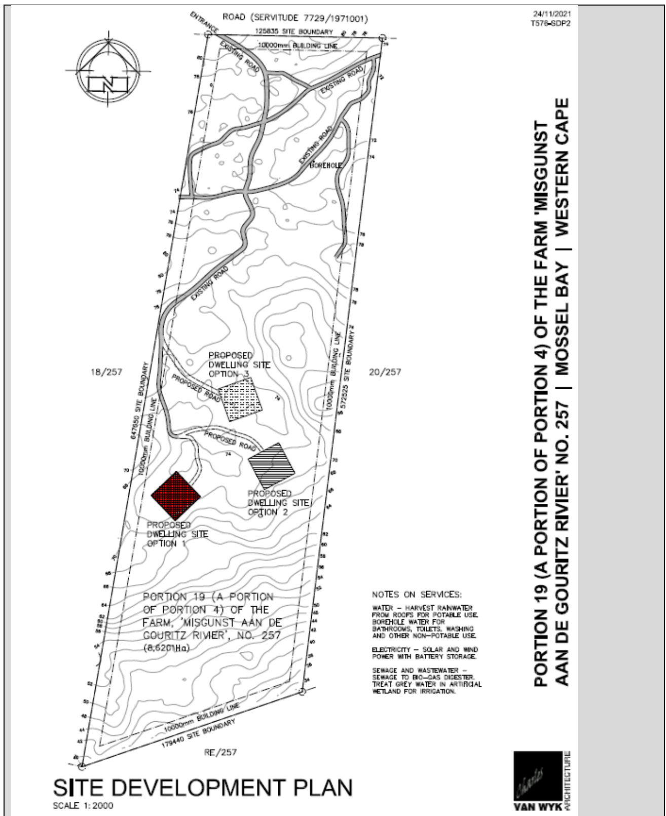
Figure 19: Site Development Plan (Option 1)
